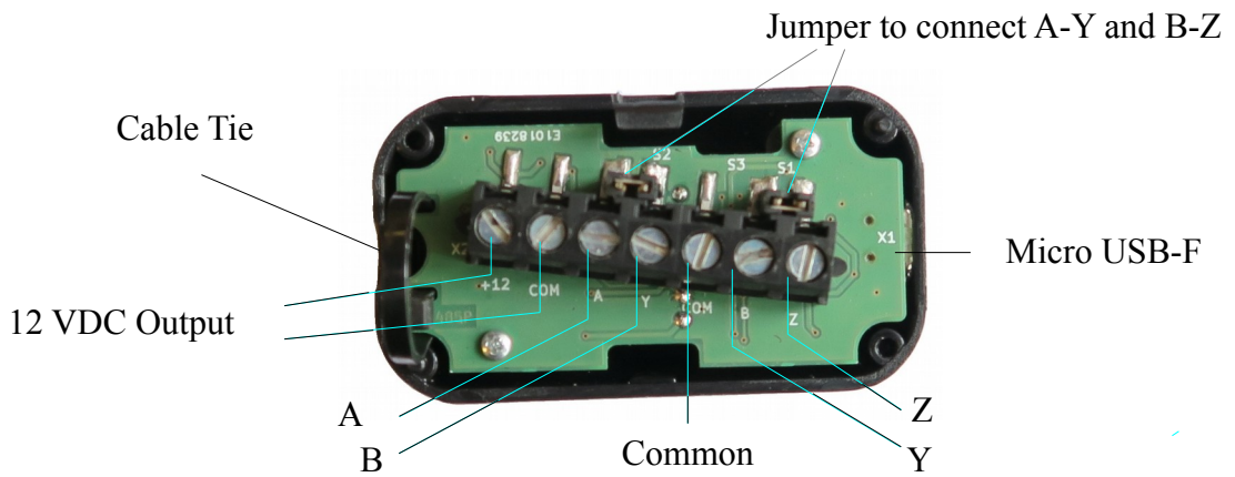
Fig. 1. Open lid converter. Connectors
