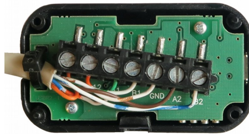
Fig. 2. Cable installation
