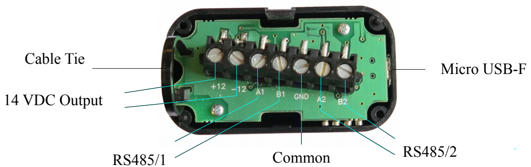
Fig. 1. Open lid converter. Connectors
